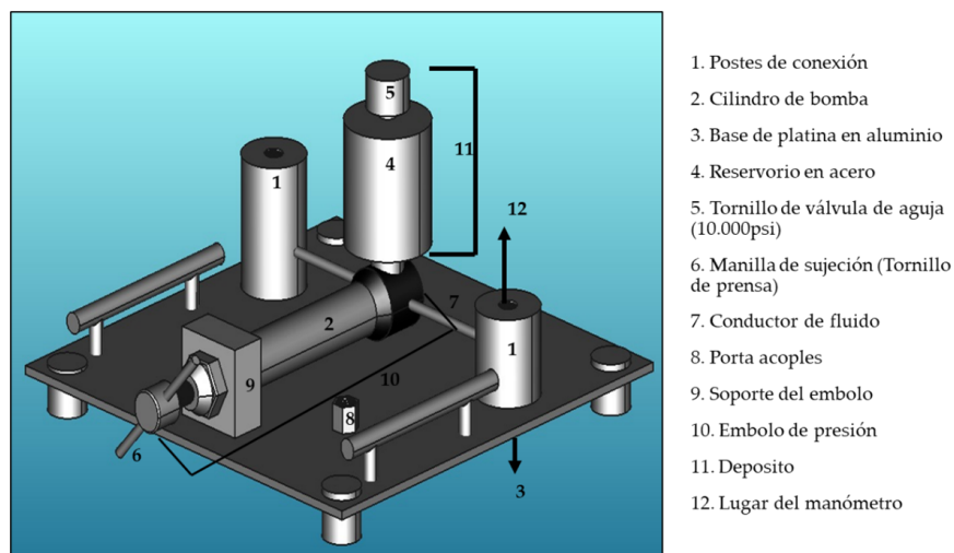
Figure 3. Plan of the test bench prototype.
