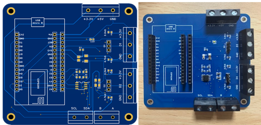
Figure 7. PCB design and actual image of the sensor and data acquisition card. Source: The authors.
