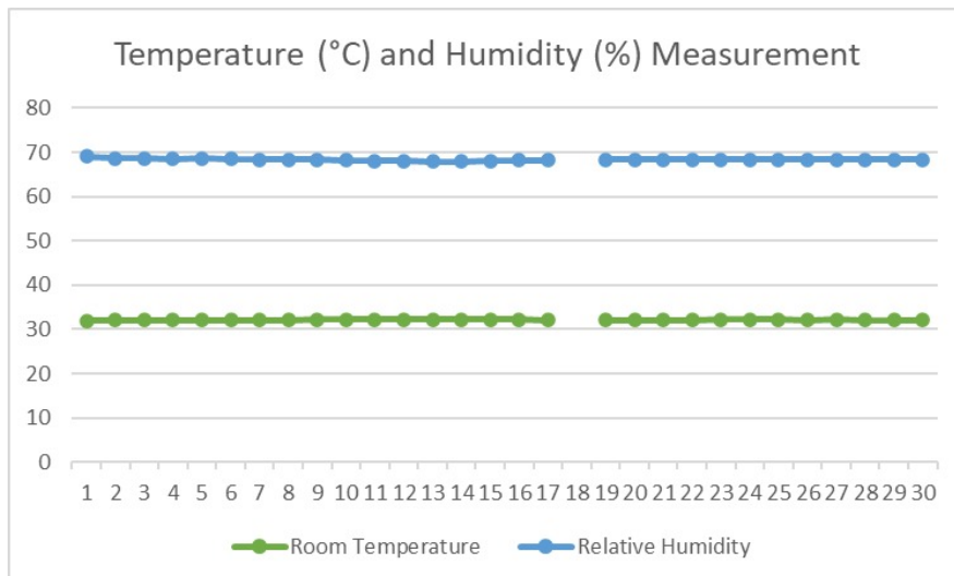
Figure 14. Capture of ambient temperature and humidity data, with a total of 29 packets received out of 30 transmitted. Transmission effectiveness of 96.67%. Source: The authors.
