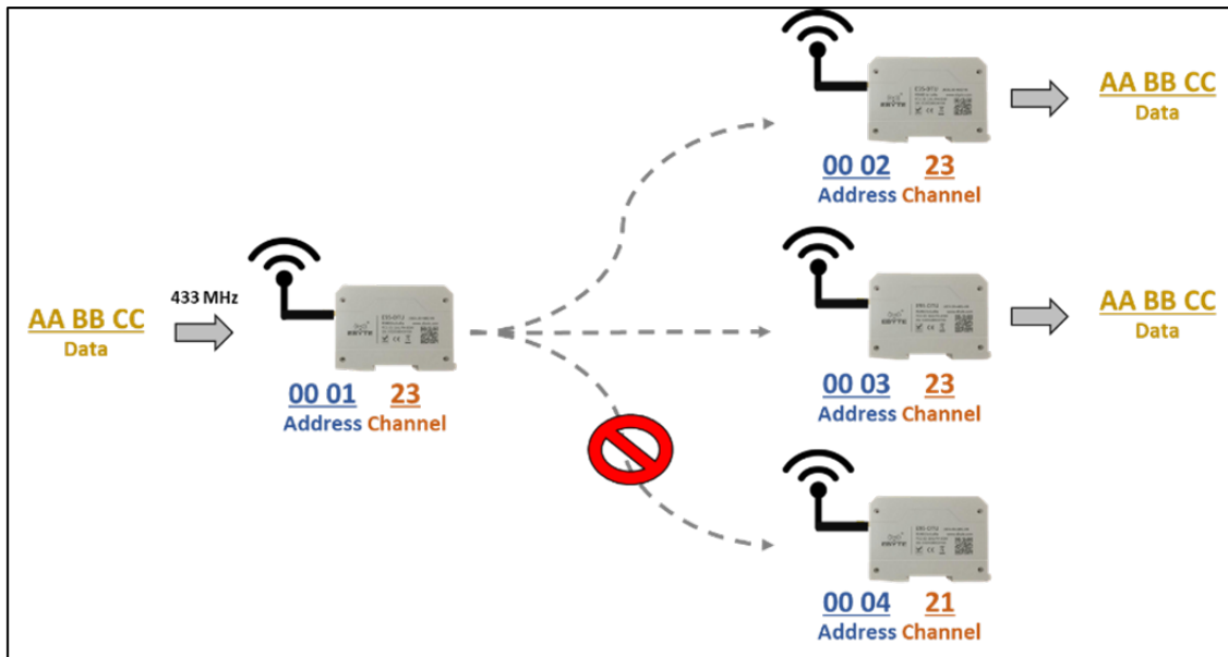
Figure 8. Configuration diagram for the transmitter and receiver nodes.
