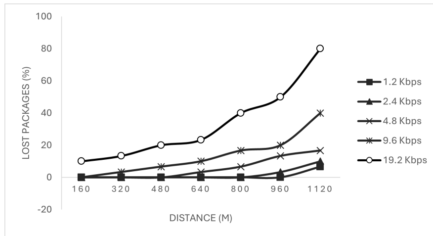
Figure 9. Percentage of packets lost by distance in meters and transmission rate configuration of the LoRa modules. Source: The authors.
