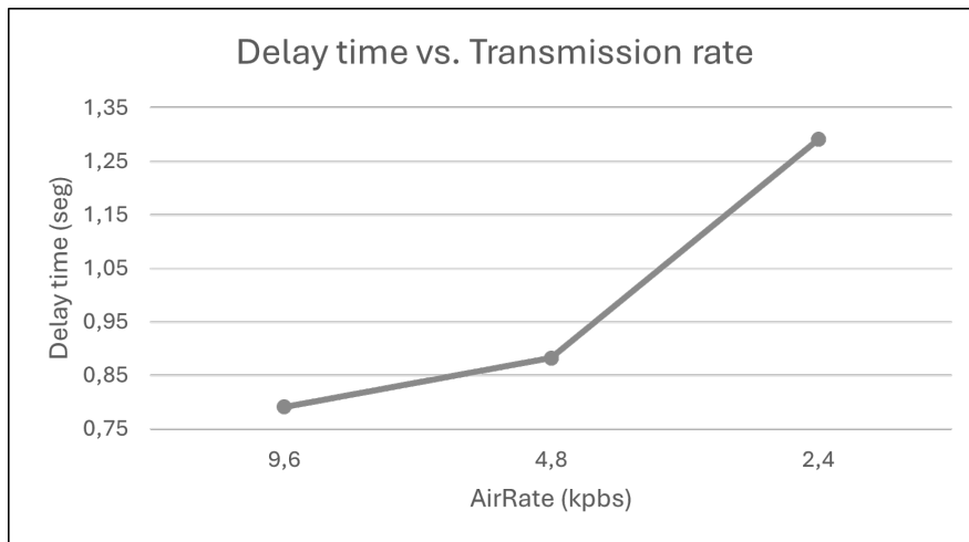
Figure 13. Delay time per transmission rate in the module configuration. Source: The authors.
