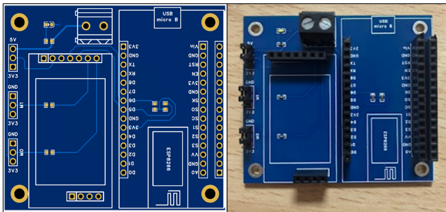
Figure 6. PCB design and actual image of the LoRa module board. Source: The authors.
